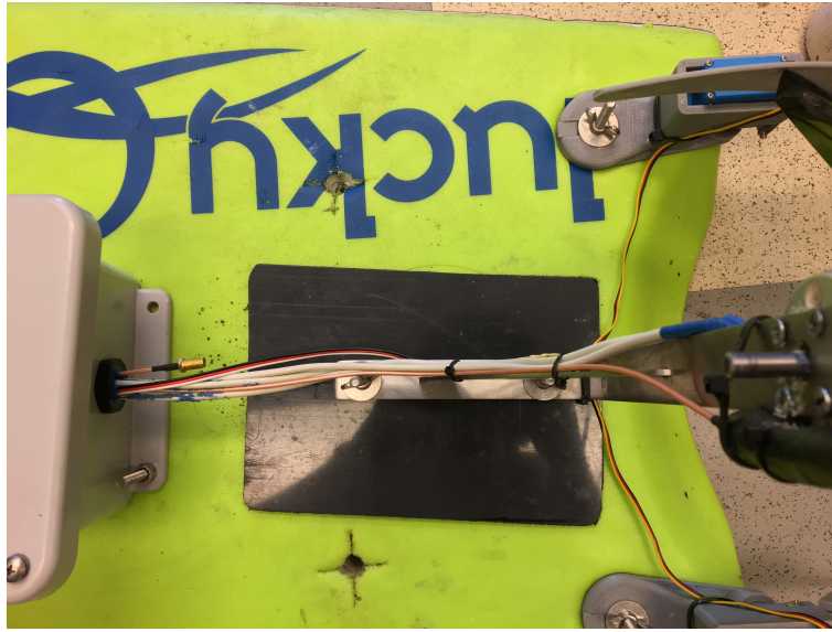
Figure 7: Ensure that all wires are present in their correct lengths. Additionally, check that the SMA cables are oriented with the correct connectors inside and outside of the bulkhead.
